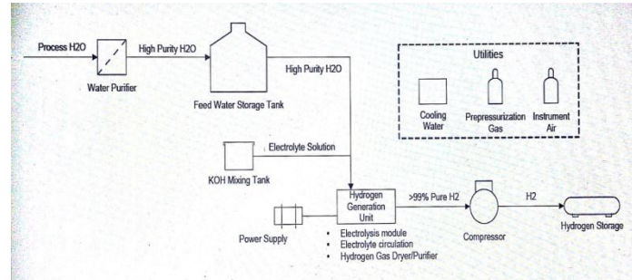
Figure 1: Process Flow Diagram
