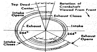
Figure 4: Valve Timing Diagram
