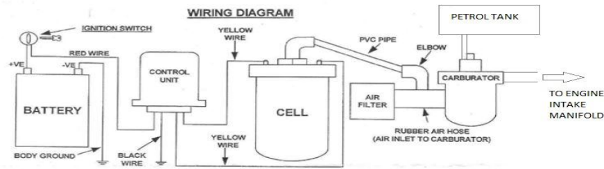
Figure 9: Arrangement of SI engine with HHO kit
