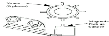
Figure 5: View Distributor Vanes
