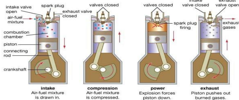
Figure 2: Cross-section schematic of a four stroke SI engine
