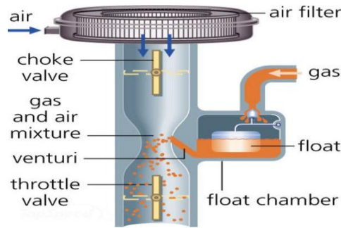
Figure 3: Cross section of a single barrel carburetor
