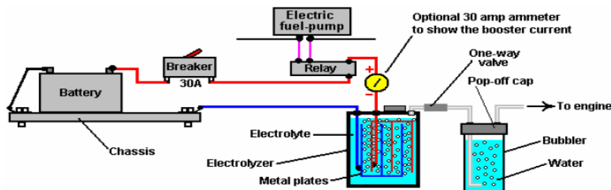
Figure 6: Electrolysis process for hydrogen generation
