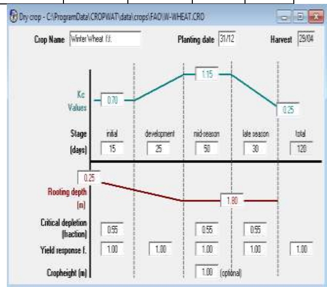
Fig. 2 Kc curve and Crop Growth stages
