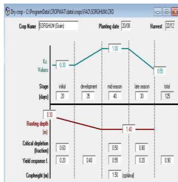
Fig. 7 K_c curve and crop growth stage
