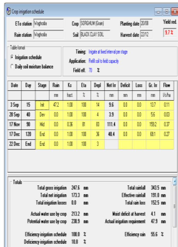
Fig.10 Computation of Irrigation Scheduling of Sorghum
