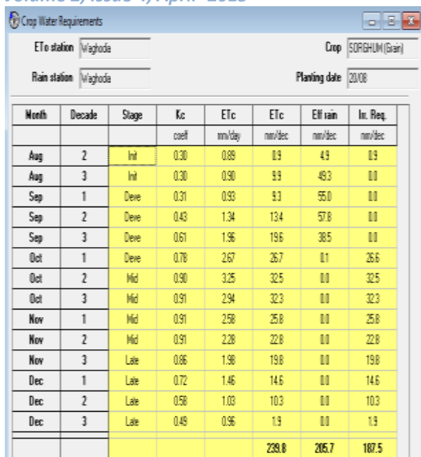
Fig 9 Crop water requirement of Sorghum
