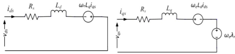
"Figure 3 Steady state PMSG model in the rotor reference frame"
