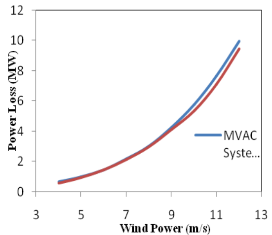
"Figure 5 Real power losses"
