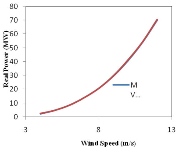
"Figure4 Real Power Generated"
