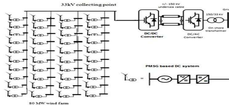
"Figure 2 MVDC offshore wind farm distribution system connected to the grid"
