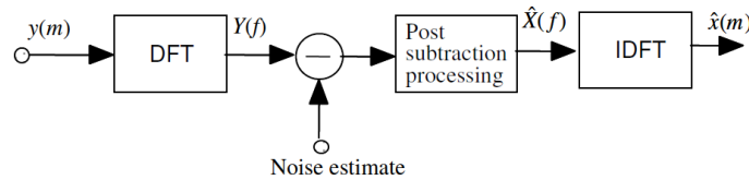
Fig.1 A block diagram illustration of spectral subtraction [15].
