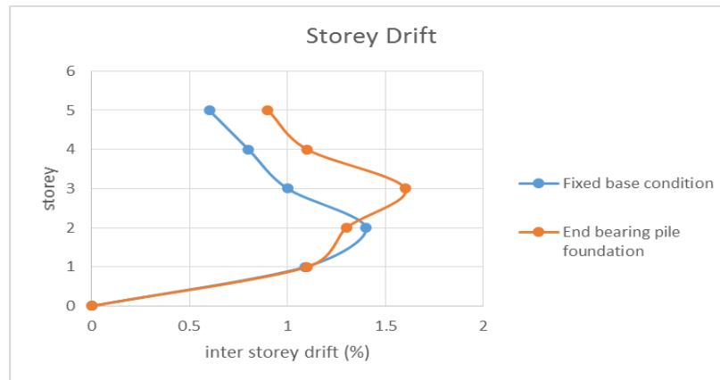
Figure 4. Aaverage experimental inter storey drift: (a) fixed base structure (b) structure supported on end baering pile foundation
