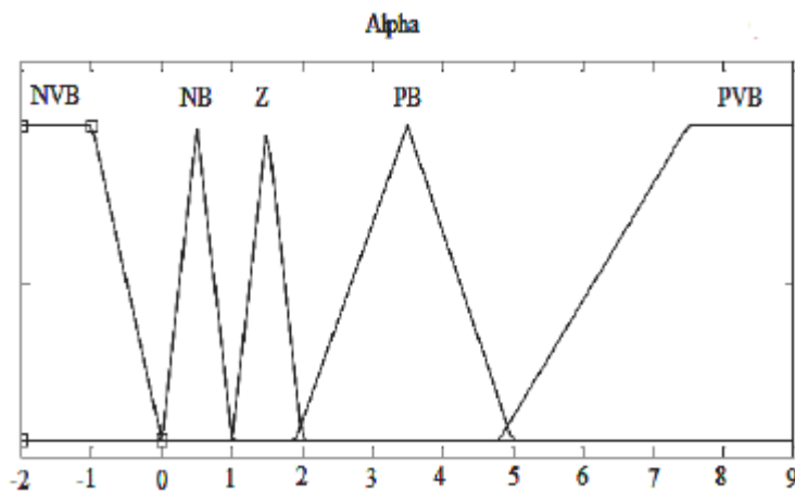
“Figure 5. Output Membership function of \alpha ”
