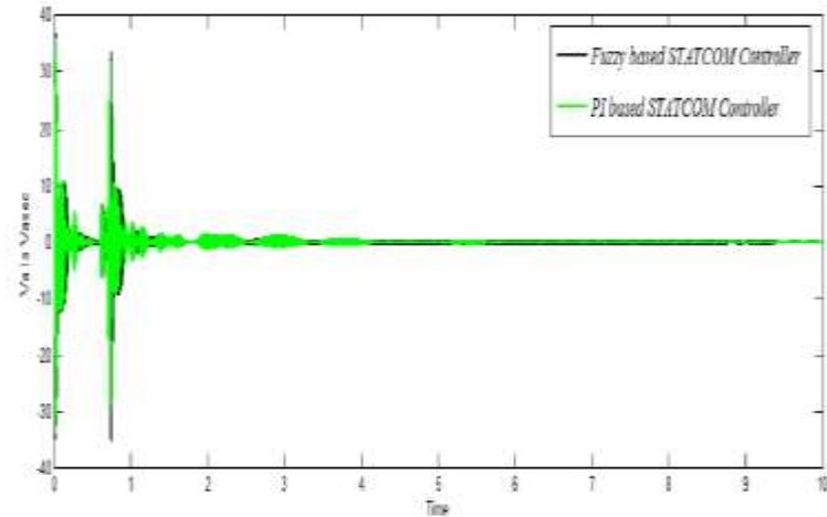
“Fig 11. Variation of Vasec Va1a with time”
