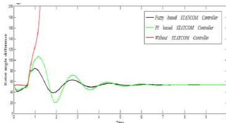
“Fig 7. Rotor angle difference with time”
