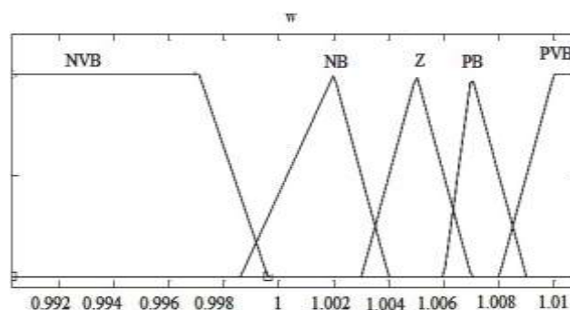
“Figure 3. Input Membership function of \omega ”
