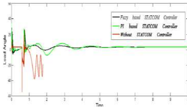
“Fig 8. Load angle with time”
