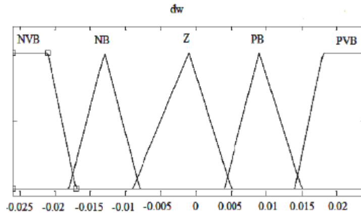
“Figure 4. Input Membership function of d\omega/dt ”
