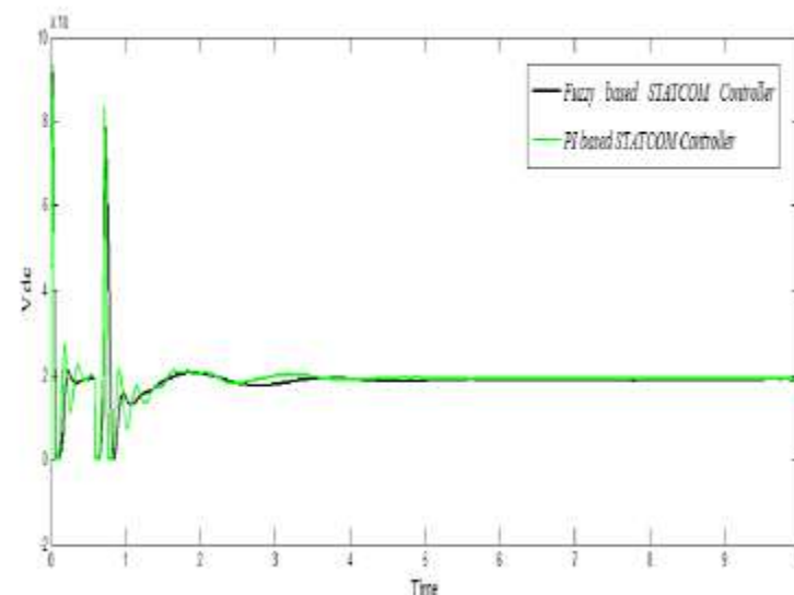
“Fig 10. Variation of Vdc with respect to time”
