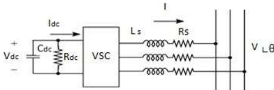
“Figure 1. STATCOM's Basic Circuit Diagram”
