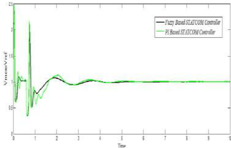
“Fig 12. Variation of Vmeas Vref with time”
