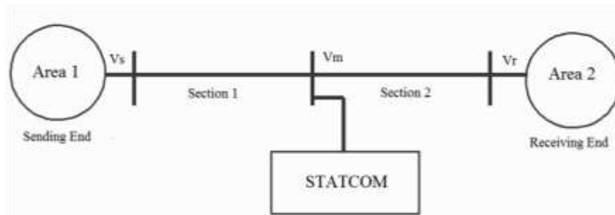
“Figure 2. Single line diagram of two area interconnected system”
