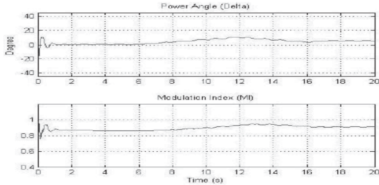
Figure 5: Simulated delta and modulation index of the 11-level inverter.
