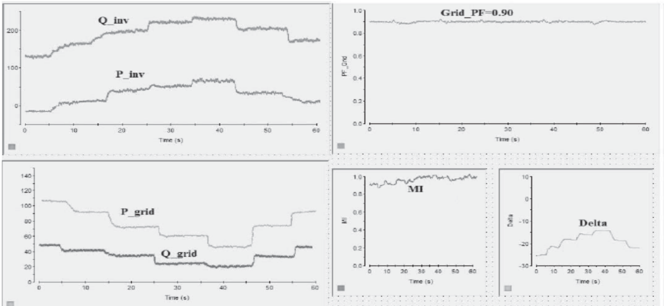
Figure 6: System parameters where the inverter is connected to the grid. (a) When wind speed is zero and there is no active power coming from wind emulator. (b) When wind speed is changing and the incoming active power from the wind emulator is changing.
