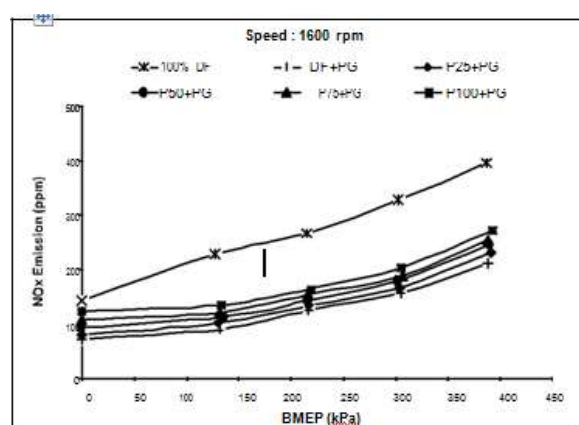
Fig. 7: Effect of BMEP on NOx Emission
