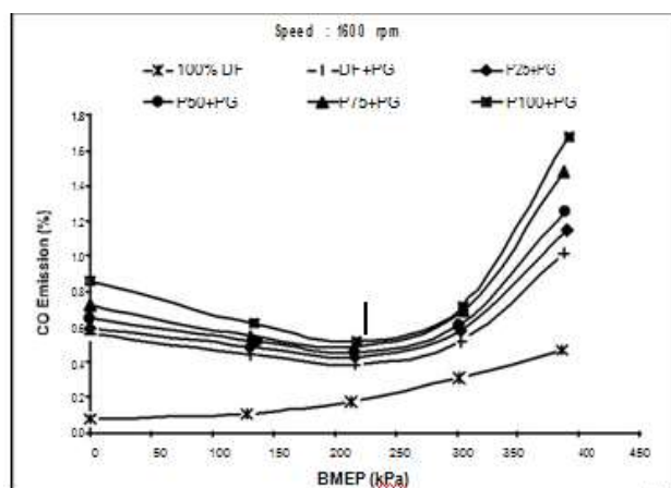
Fig. 6: Effect of BMEP on CO Emission
