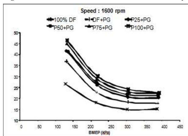
Fig. 4: Effect of BMEP on Specific Energy Consumption
