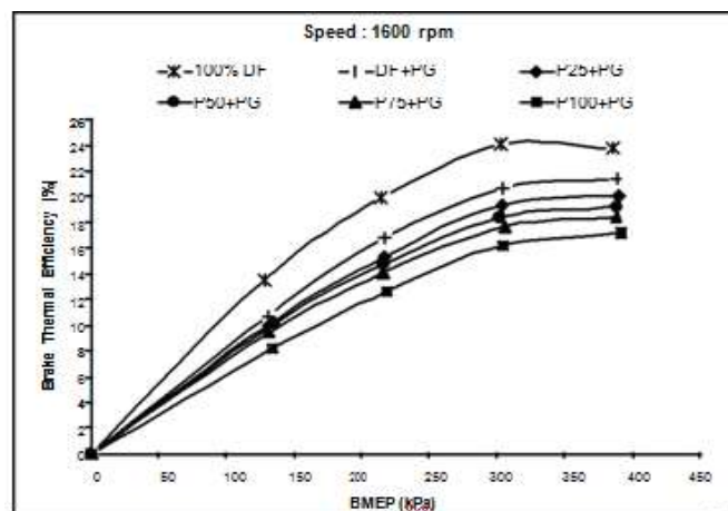
Fig. 3: Effect of BMEP on Brake Thermal Efficiency
