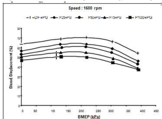
Fig. 5: Effect of BMEP on Diesel Displacement
