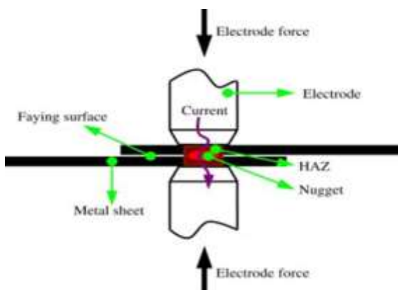
Fig: 1 Spot Welding
