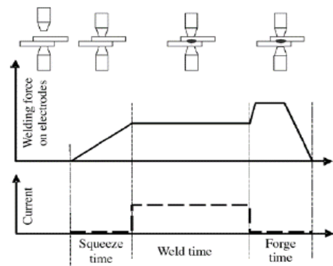
Fig: 2 Spot welding cycle
