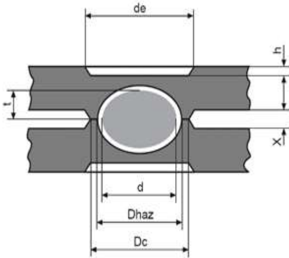
Fig: 3 Dimension of nugget
