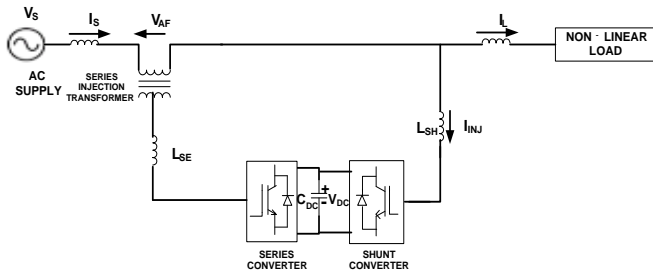
Figure 1. Line diagram of unified power quality conditioner
