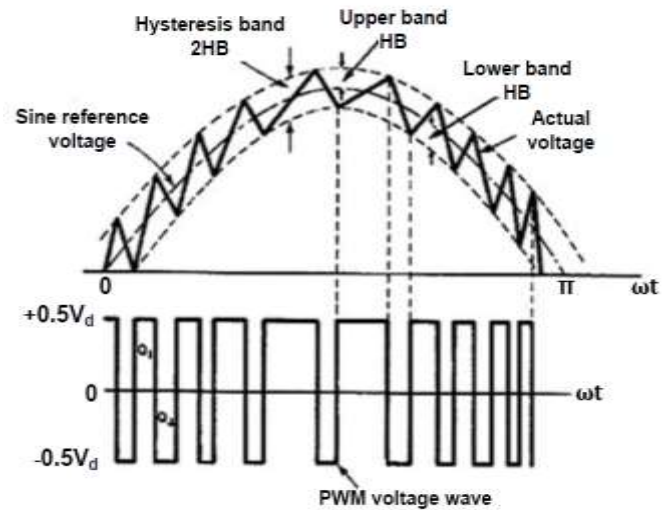
Figure 8. Hysteresis voltage control technique
