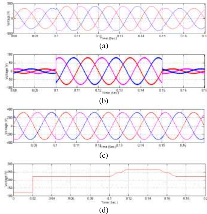
Figure 19. Voltage Swell Condition (a) Source Voltage (b) Transformer Injected Voltage (c) Load Voltage (d) RMS Value
