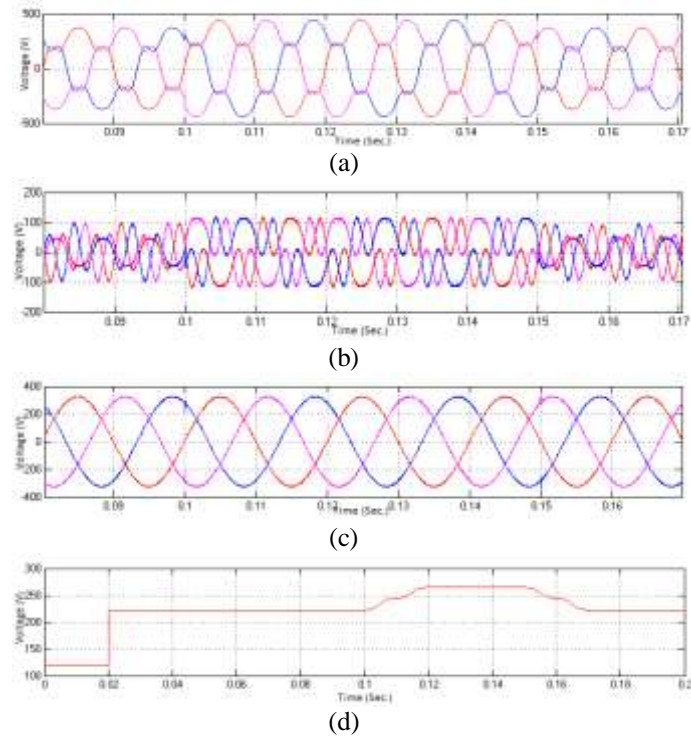
Figure 22. Voltage Swell with Harmonics Distortion Condition (a) Source Voltage (b) Transformer Injected Voltage (c) Load Voltage (d) RMS Value
