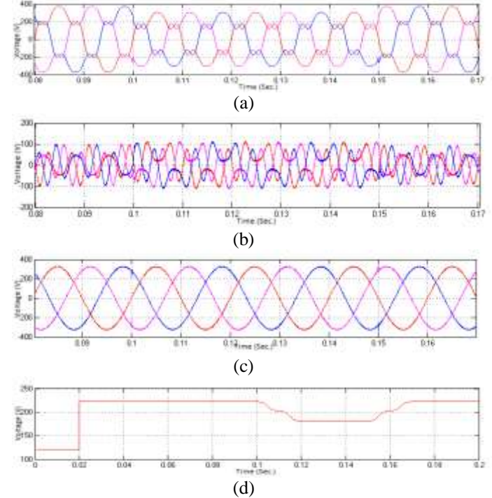
Figure 21. Voltage Sag with Harmonics Distortion Condition (a) Source Voltage (b) Transformer Injected Voltage (c) Load Voltage (d) RMS Value
