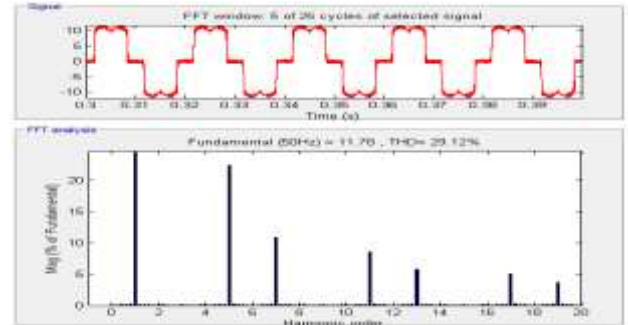
Figure 25.THD=29.12 % of Load Current
