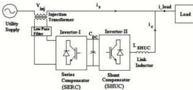
Figure 2. Right Shunt UPQC Structure
