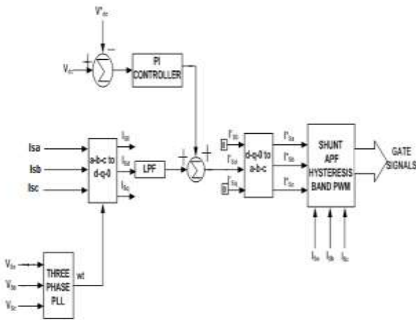
Figure 7. Control block diagram of d-q theory in shunt active filter
