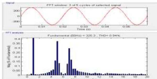
Figure 24. THD=0.94% of Source voltage
