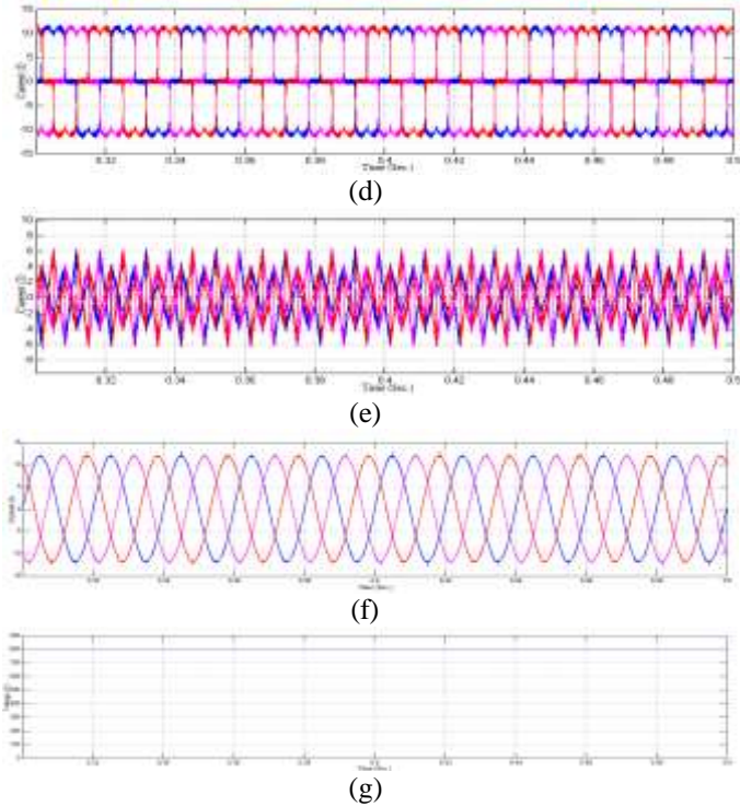
Figure 15. Balanced Voltage Condition (a) Source Voltage (b) Transformer Injected Voltage (c) Load Voltage (d) Load Current (e) Shunt APF Injected Current (f) Source Current (g) DC Source Voltage
