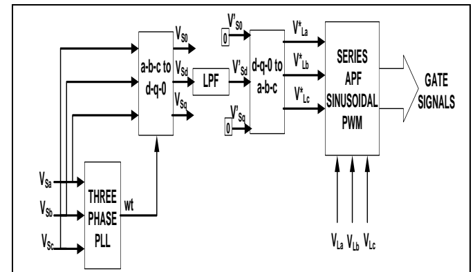
Figure 6. Control block diagram of d-q theory of Series APF
