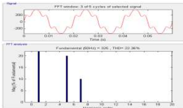
Figure 23. THD=22.36% of Source voltage
