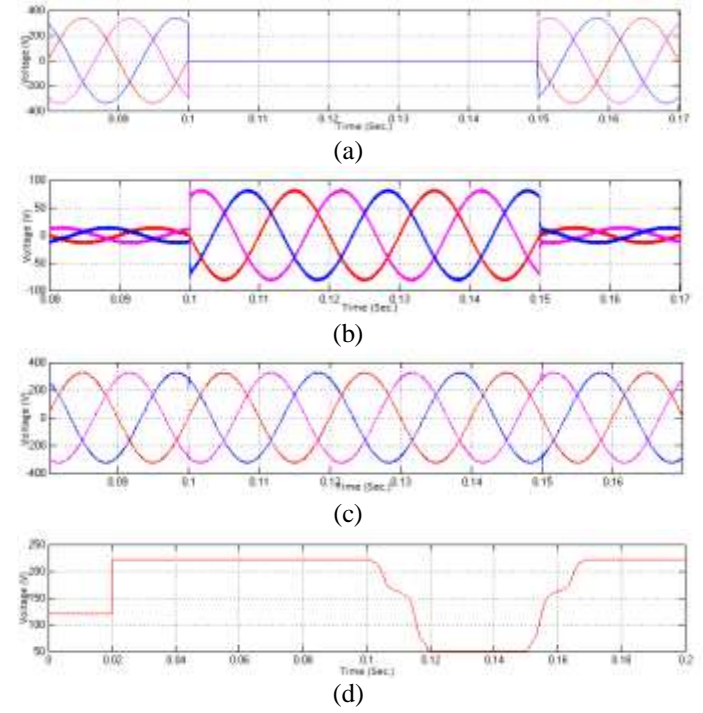
Figure 20. Voltage Interruption Condition (a) Source Voltage (b) Transformer Injected Voltage (c) Load Voltage (d) RMS Value
