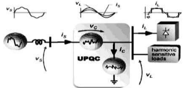
Figure 13. Basic block diagram of unified power quality conditioner
