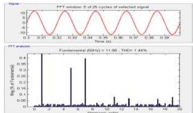
Figure 26.THD=1.44 % of Source Current
