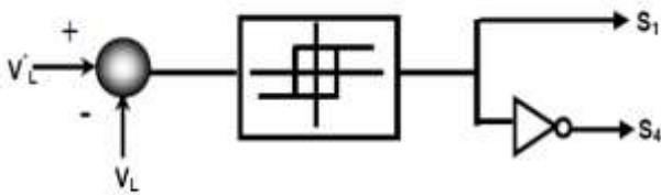
Figure 9. Control block of hysteresis band voltage control technique
