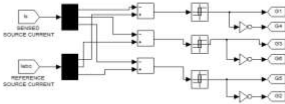
Figure 12. Simulink diagram of hysteresis current controller
