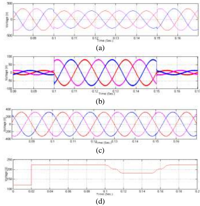
Figure 18. Voltage Sag Condition (a) Source Voltage (b) Transformer Injected Voltage (c) Load Voltage (d) RMS Value
