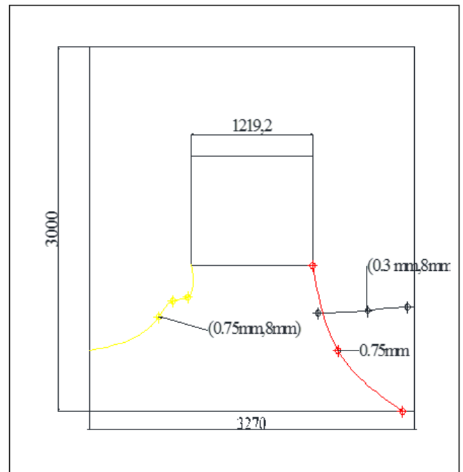
Figure: 8 Crack profile for Master bedroom wall 1
