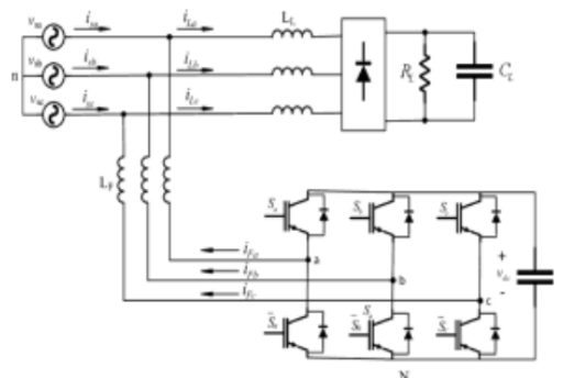
Fig.1 Three phase active power filter
