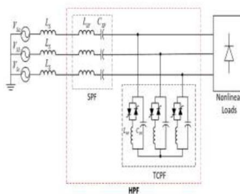
Fig.3 Configuration of the hybrid power filter
