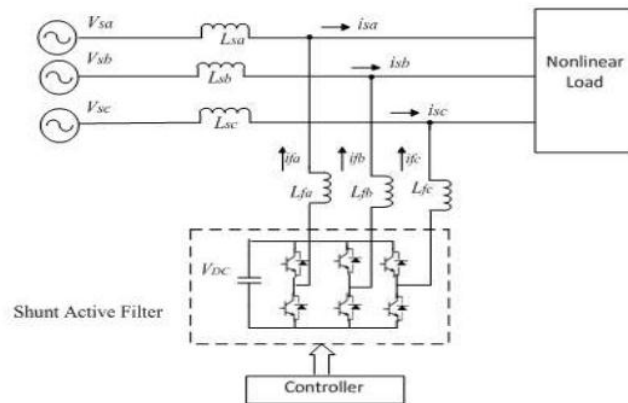
Fig.2 Configuration of conventional APF
