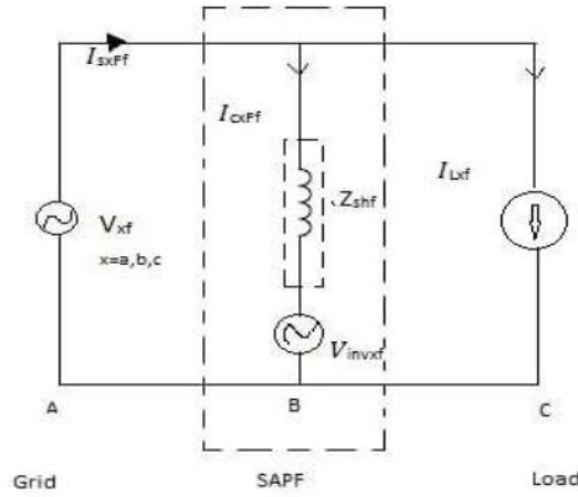
Fig.5 Fundamental equivalent circuit of the proposed APF system
