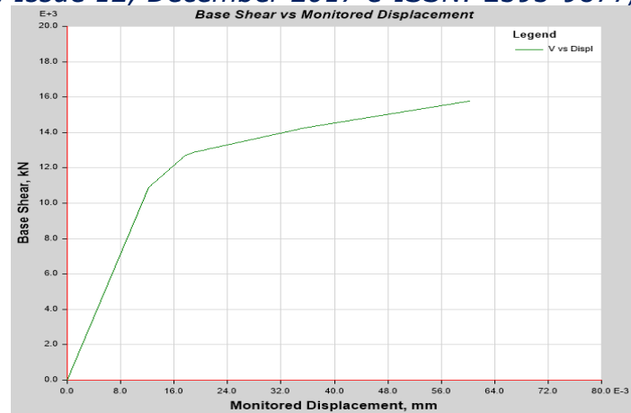
Chart -1: Output pushover curve form ETAB2016
