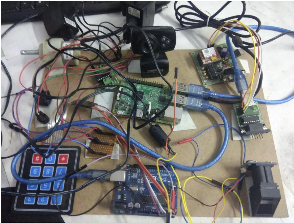
Fig.4.1 Biometric Based Lock Process For Shared Access
