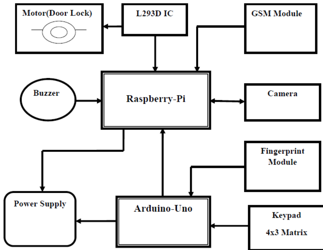
Fig. 3.1 Block Diagram
