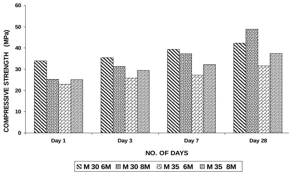
Fig. 5.1 Graphical Representation for Compressive Strength of BA and GGBS based Geopolymer Paver Block Concrete
