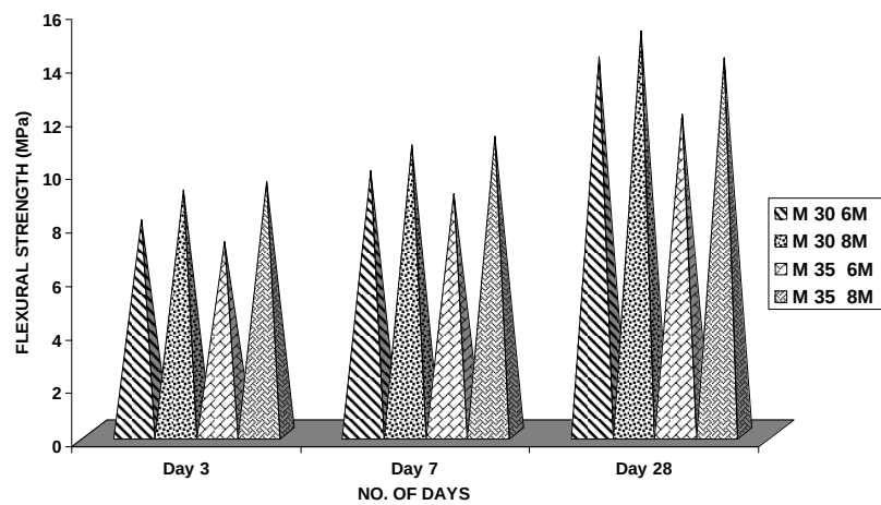
Fig. 5.2 Graphical Representation for Flexural Strength of BA and GGBS Based Geopolymer Paver Block Concrete
