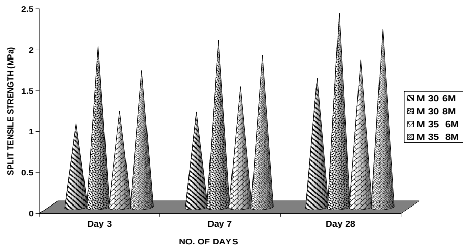
Fig. 5.3 Graphical Representation for Split Tensile Strength of BA and GGBS based geopolymer Paver Block Concrete
