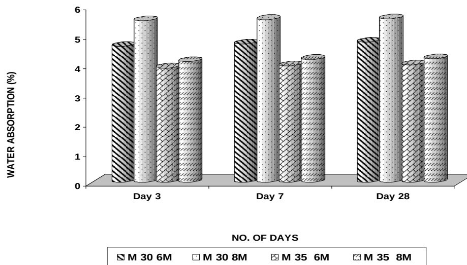
Fig. 5.4 Graphical Representation for Water Absorption of BA and GGBS Based Geopolymer Paver Block Concrete
