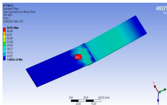
Fig 5 : Stress generated in plate (at 4000N)
