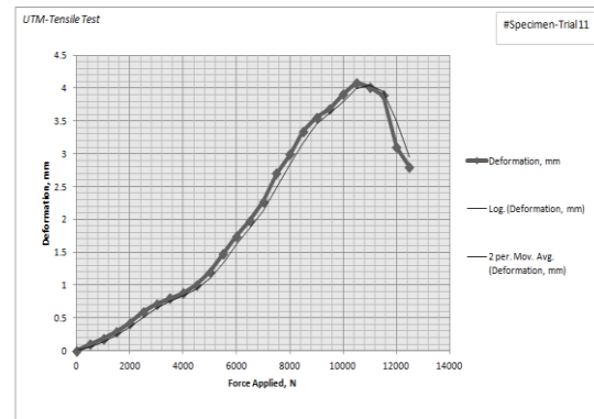
Fig 4.: Plot of Load vs. Displacement
