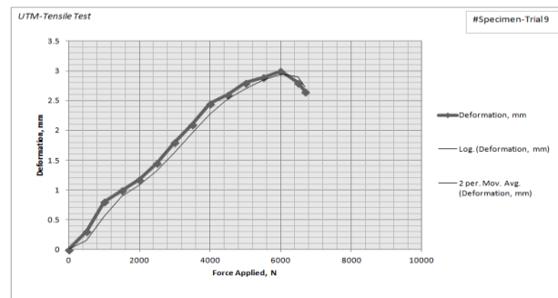
Fig.1: Plot of Load vs. Displacement
