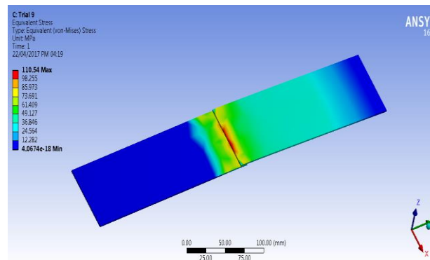
Fig 2: Stress generated in plate (at 4000N)
