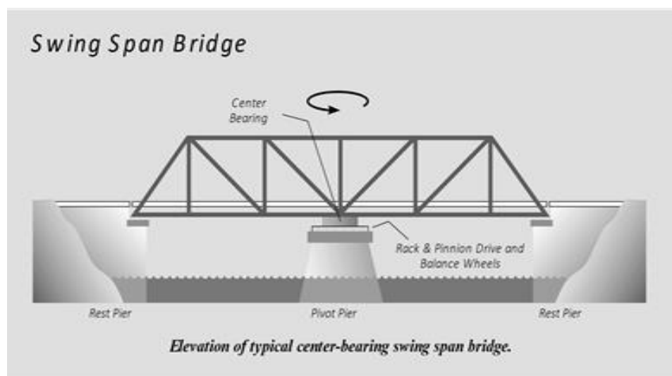
Fig.1.Elevation of Swing Span Bridge
