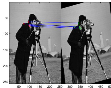
Figure 4.2 final match points
