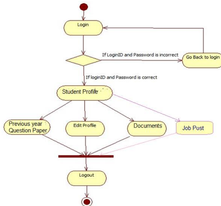
Activity Diagram for Student
