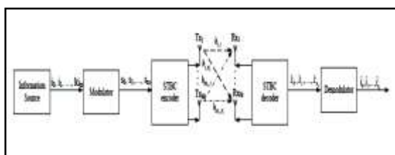
Figure 2 Generalized block diagram of STBC Communication System
