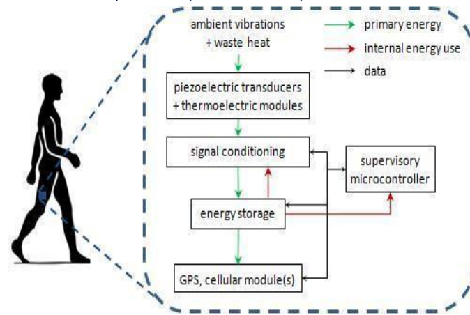
Fig. 3 Energy harvesting from human being
