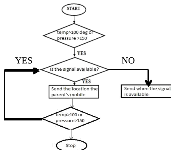
Fig.2 Working model flowchart
