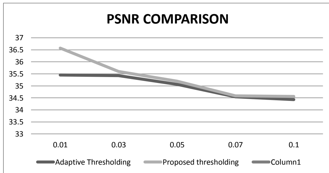
Figure (2). Graphical analysis of comparison of PSNR values for various Denoising filters
