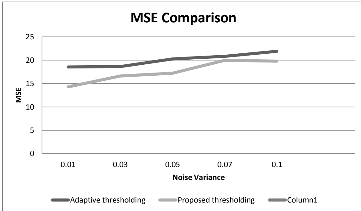
Figure (3). Graphical analysis of comparison of MSE values for various Denoising filters
