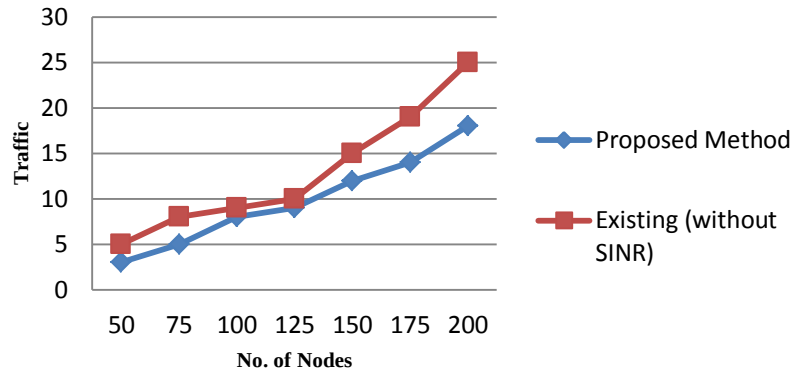
Fig.5 Average relaying traffic on each node for different data gathering strategies
