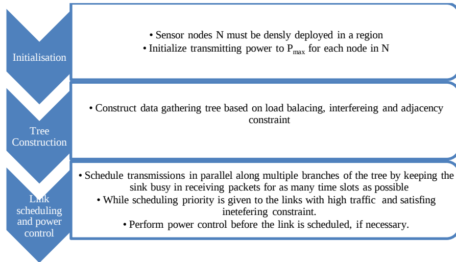
Figure 1. Flowchart of Operation of Low latency SINR based data gathering in cluster based WSN
