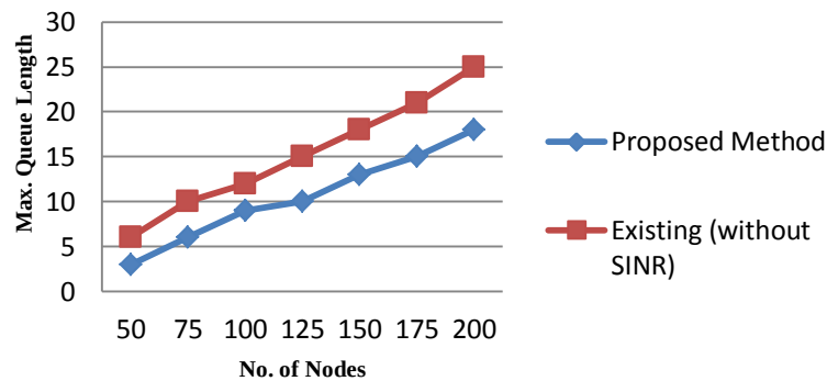
Fig 6 Maximum queue length on each node for different data gathering strategies
