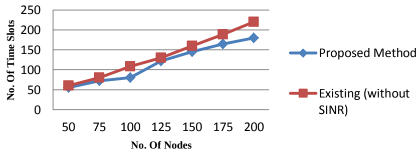
Fig 4: Number of required number of time slots for data gathering under different node densities
